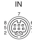
VISCA RS-232C
